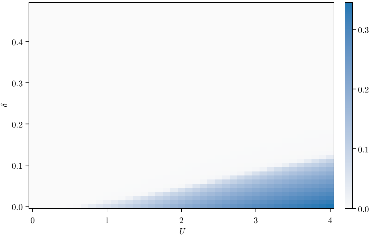
Magnetization ( t = 1.0 , V = 0.0 , L = 128 , \beta = 100.0 )
